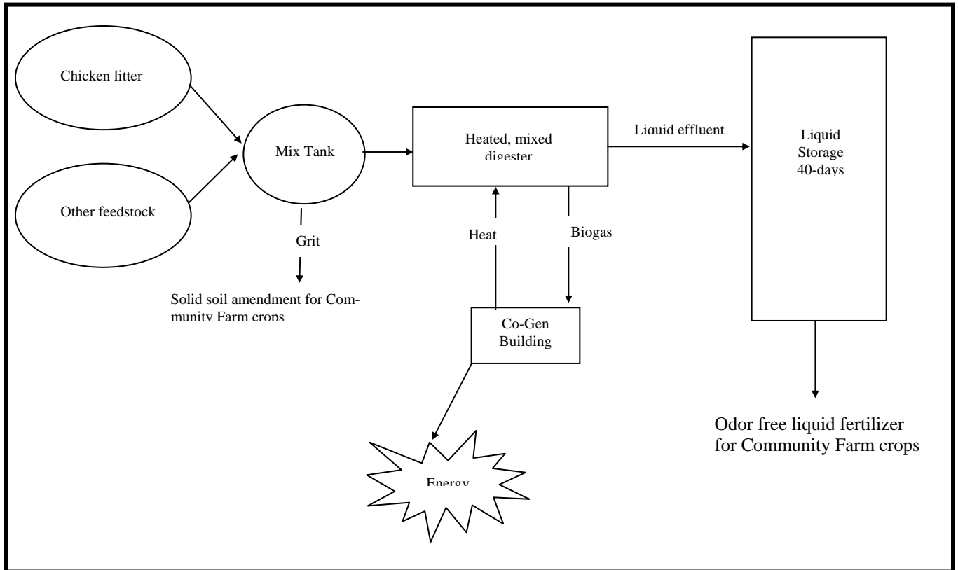
Figure 1 CONCEPTUAL DIGESTER PROCESS FLOW
