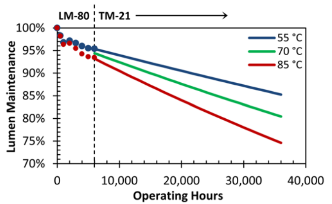
Figure 1. TM-21 extrapolation from LM-80 data.
