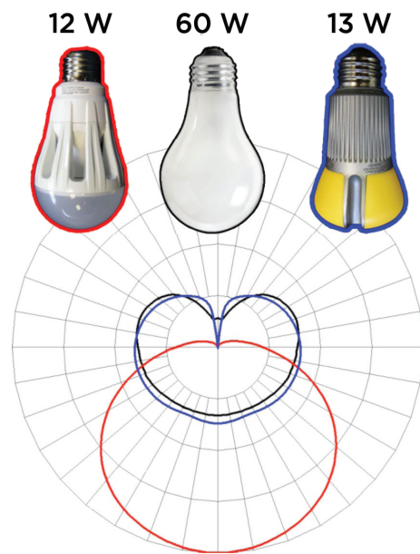
Figure 2. Distribution equivalency
