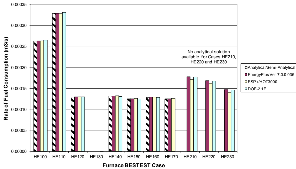
Figure 7 Rate of Fuel Consumption Results for Various Programs
