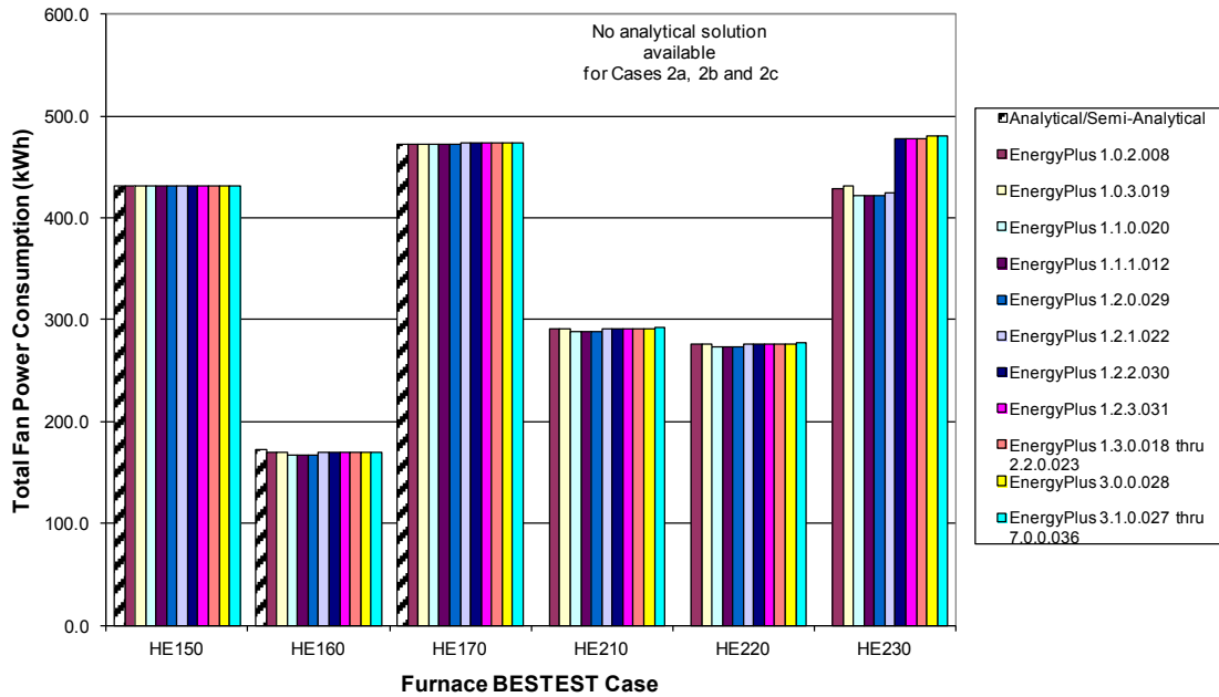
Figure 5 Total Fan Power Results for Various Release Versions of EnergyPlus (An input error was corrected for Case HE230 with version 1.2.2.032 once NREL report was released and results from other programs were available to compare to.)
