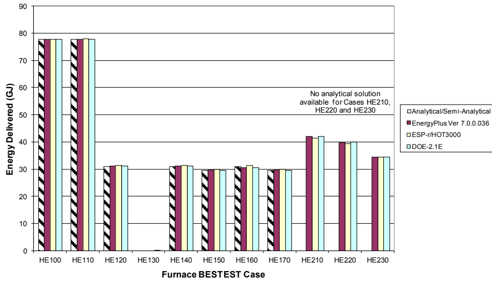
Figure 6 Energy Delivered to Space Results for Various Programs
