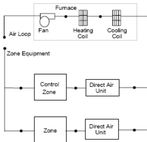
Figure 2 EnergyPlus Furnace Model
