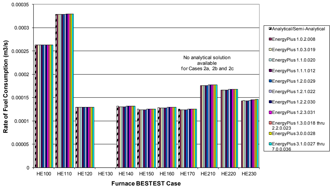
Figure 4 Rate of Fuel Consumption Results for Various Release Versions of EnergyPlus
